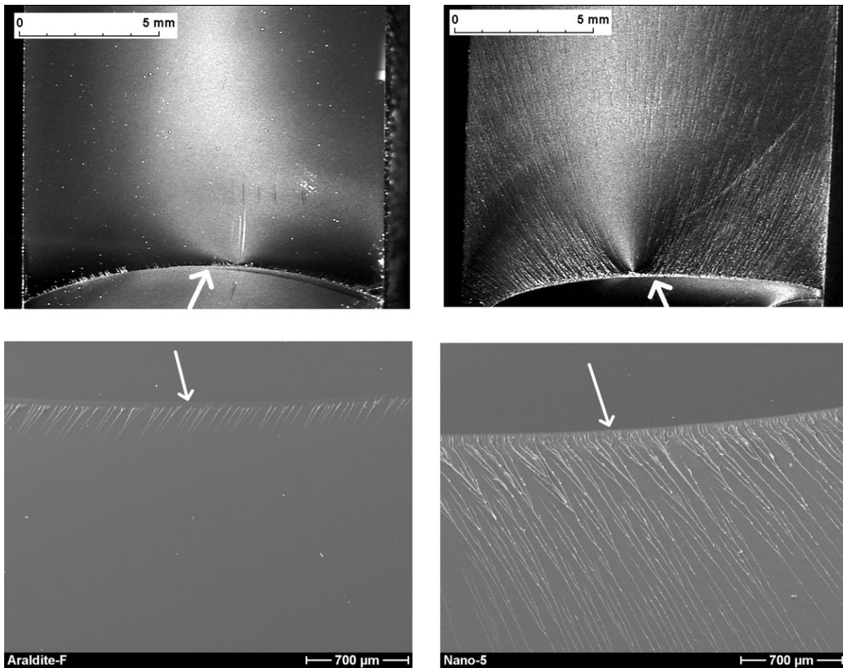
Figure 4. Fracture surfaces after crack opening of CT-samples; left: Araldite-F, right: nano SiO 2 -reinforced.
